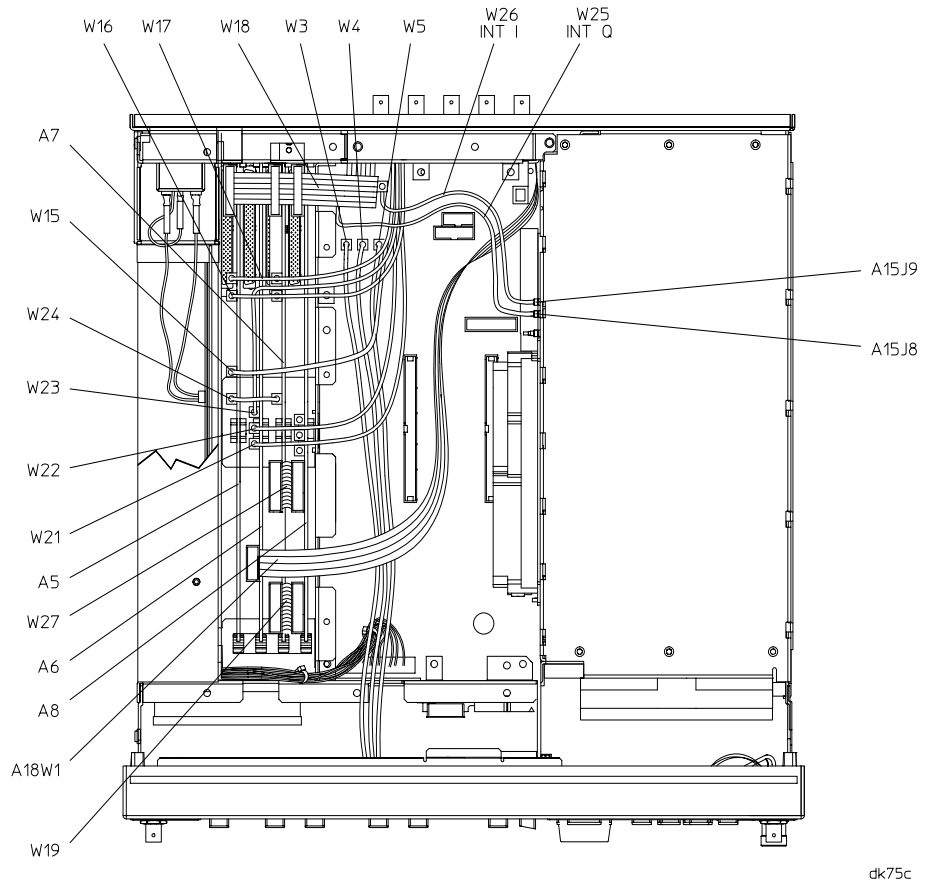
Figure 9 Cables W25 and W26
